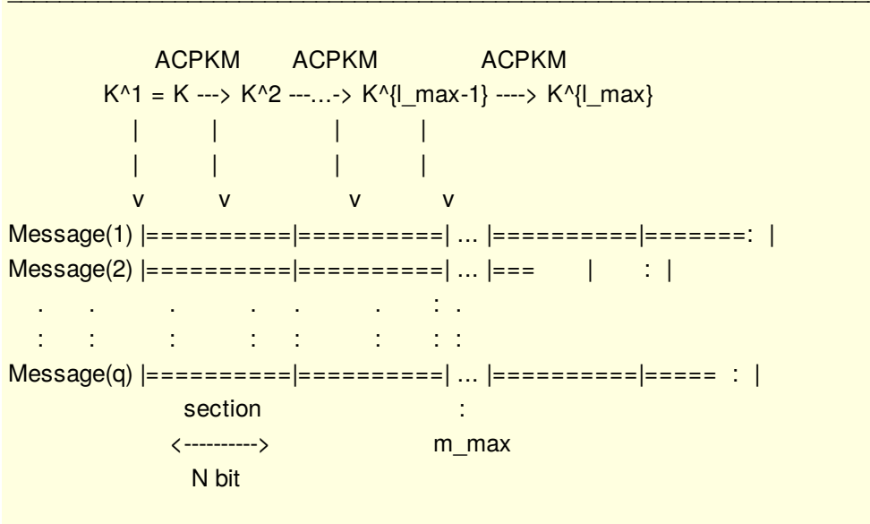
Figure 3: Key meshing with no master key
